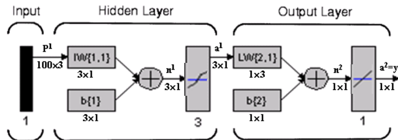
Fig. 11: Backpropagation network architecture
