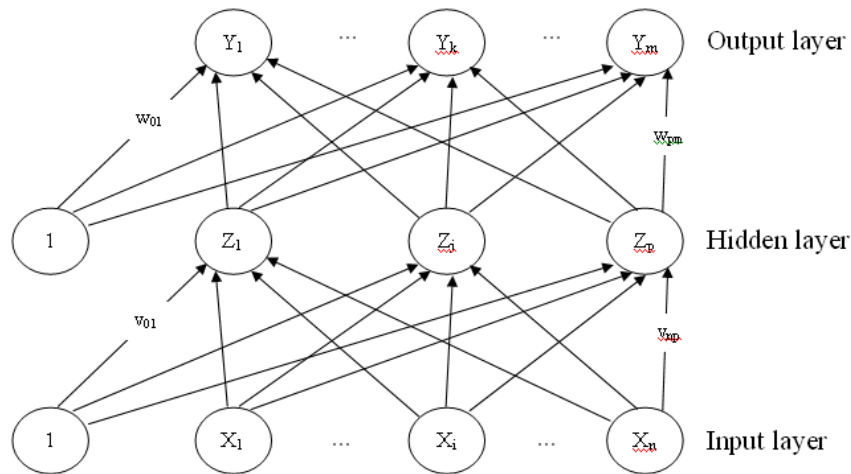
Figure (8): Backpropagation neural network with one hidden layer.
