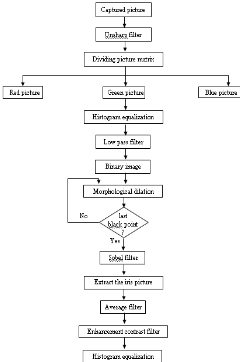
Figure (5): The block diagram of the steps adopted in the analysis of the eye image
